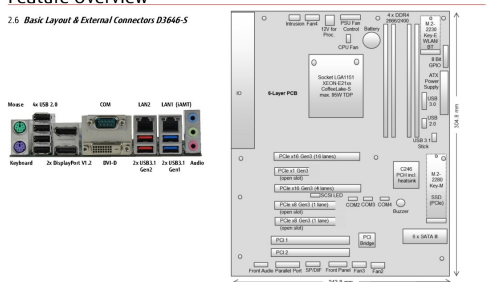
2.6 Basic Layout & External Connectors D3646-S
