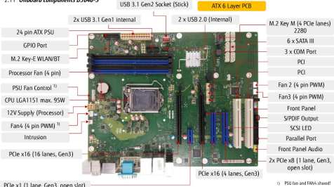
2.11 Onboard components D3646-S
