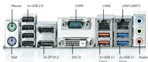
2.6 Basic Layout & External Connectors D3646-S
